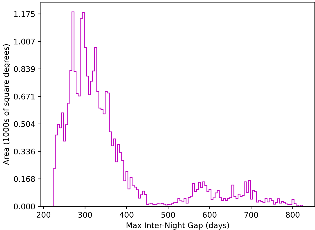
too_elab_r64_d2_griz_v3.4_10yrs All sky z band: Max Inter-Night Gap
