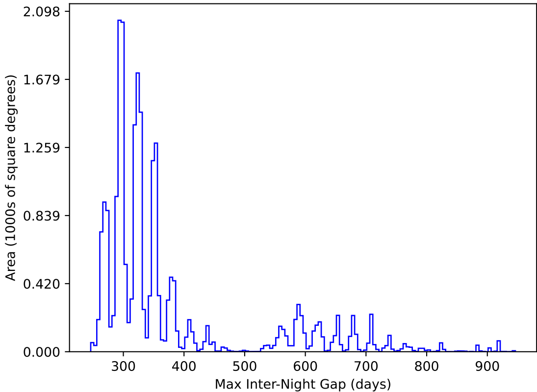
too_elab_r64_d2_griz_v3.4_10yrs All sky y band: Max Inter-Night Gap
