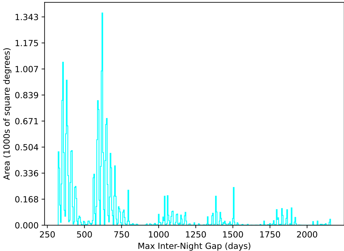
too_elab_r64_d2_griz_v3.4_10yrs All sky u band: Max Inter-Night Gap
