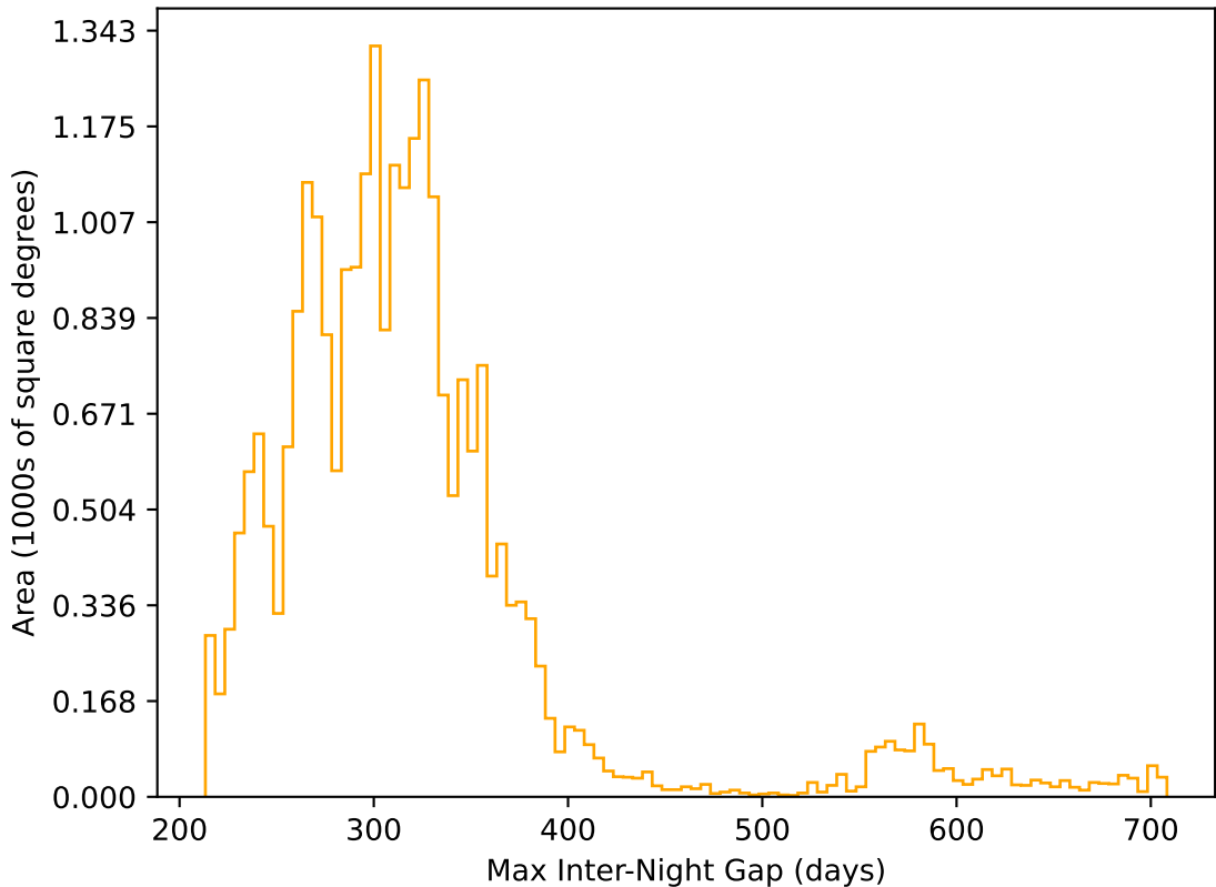
too_elab_r64_d2_griz_v3.4_10yrs All sky r band: Max Inter-Night Gap
