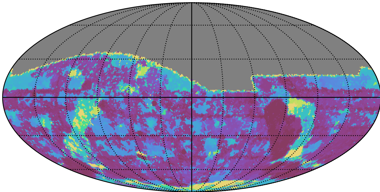
too_elab_r64_d2_griz_v3.4_10yrs All sky g band: Max Inter-Night Gap
