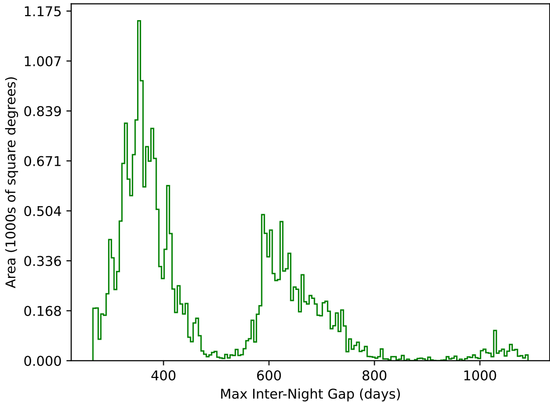
too_elab_r64_d2_griz_v3.4_10yrs All sky g band: Max Inter-Night Gap
