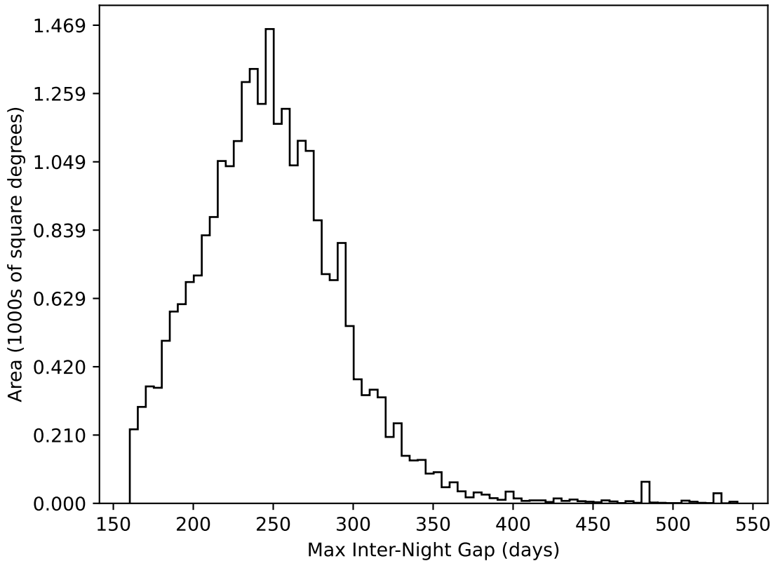
too_elab_r64_d2_griz_v3.4_10yrs All sky all bands: Max Inter-Night Gap
