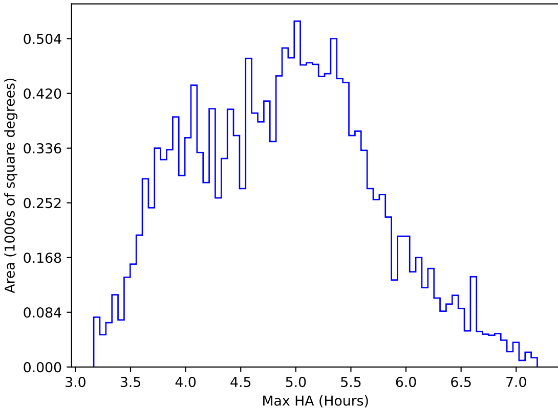
too_elab_r64_d2_griz_v3.4_10yrs WFD z band: Max HA
