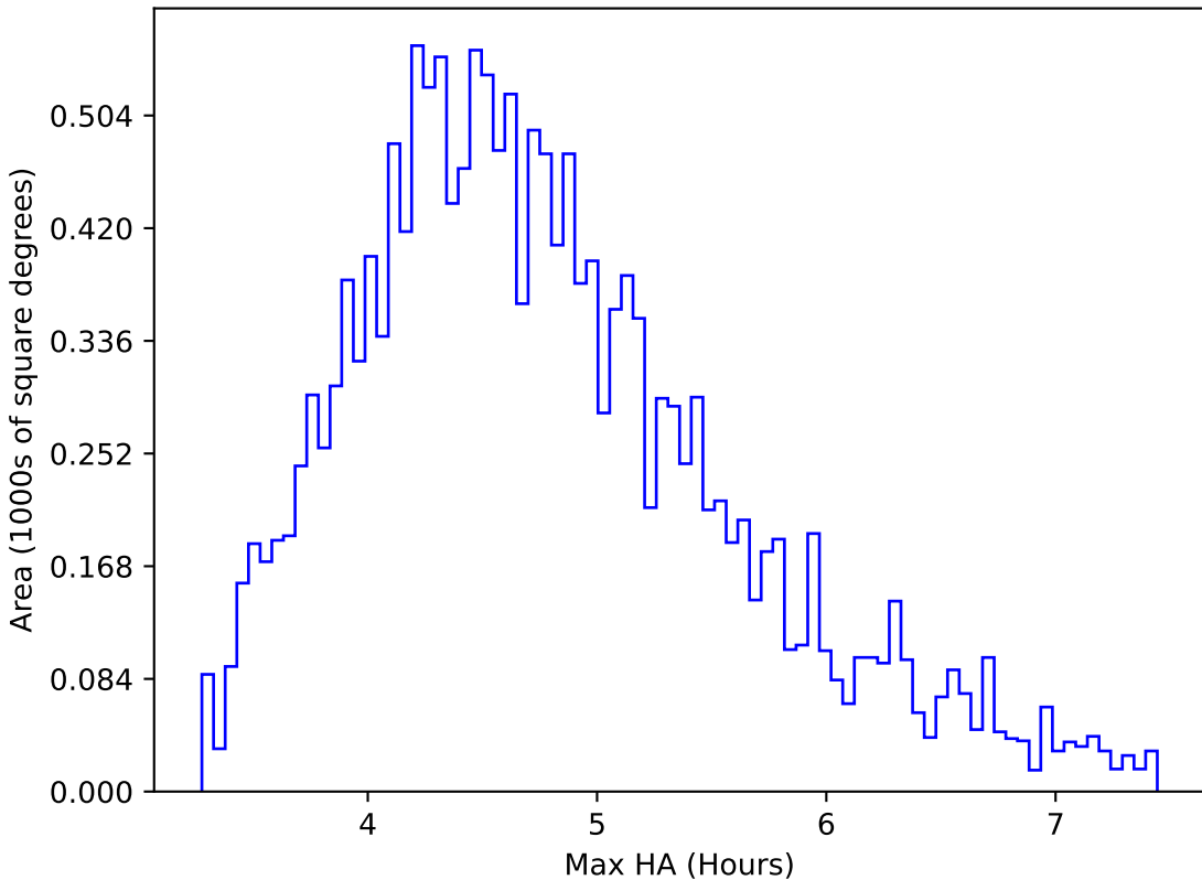
too_elab_r64_d2_griz_v3.4_10yrs WFD y band: Max HA
