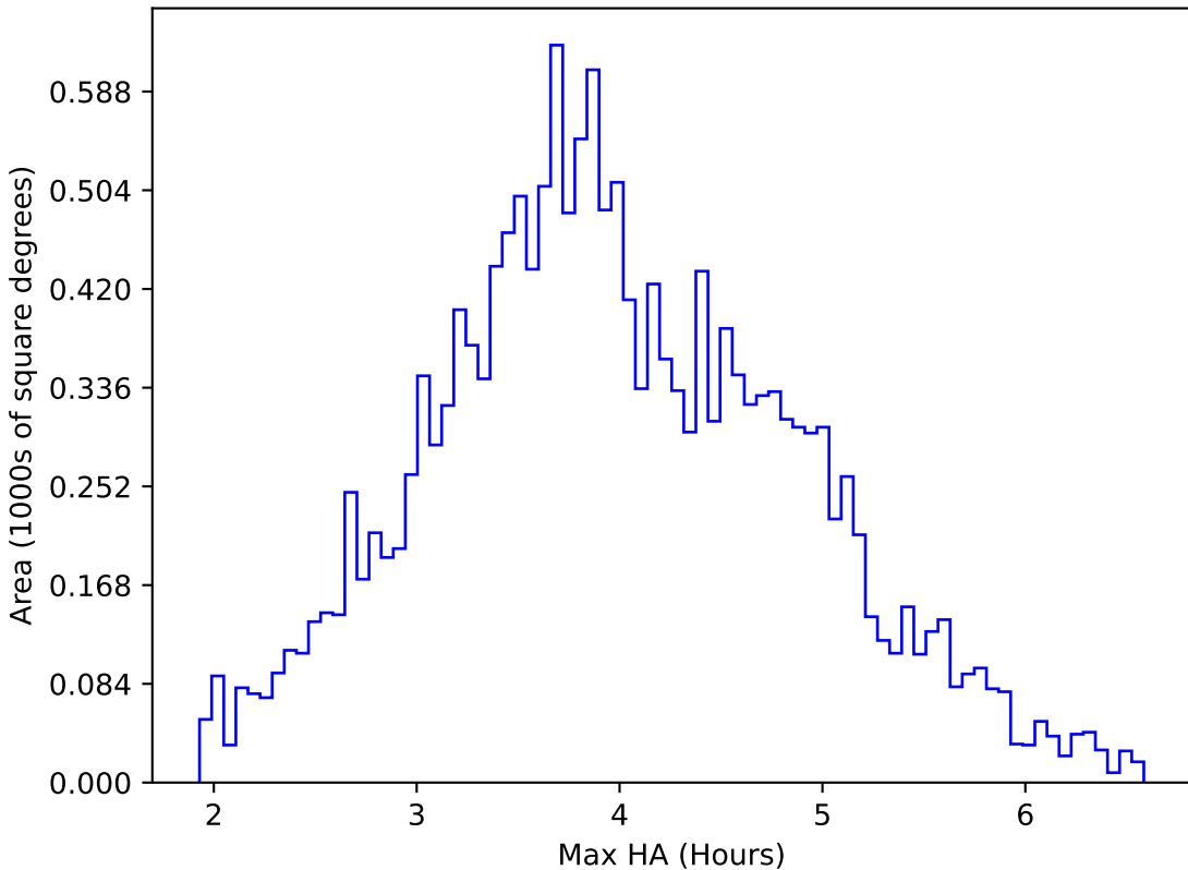
too_elab_r64_d2_griz_v3.4_10yrs WFD u band: Max HA
