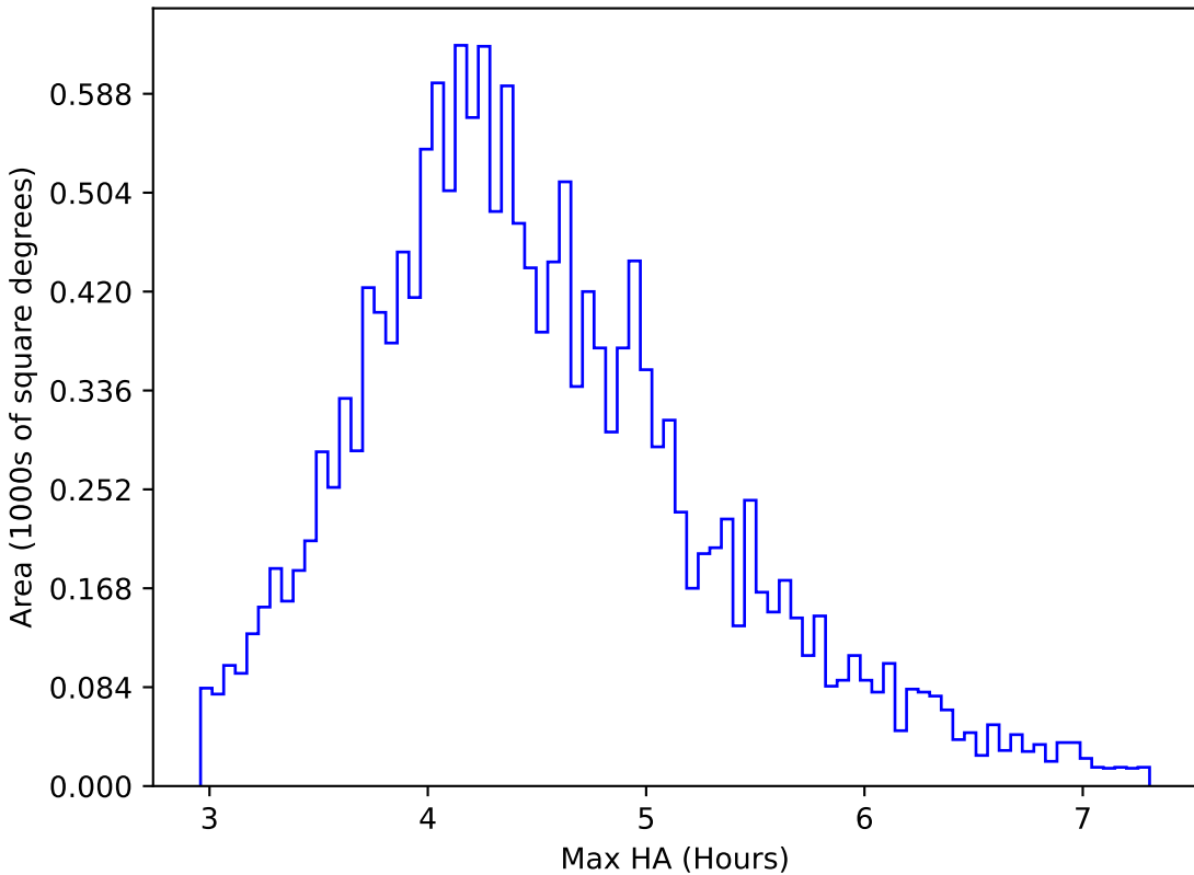
too_elab_r64_d2_griz_v3.4_10yrs WFD r band: Max HA
