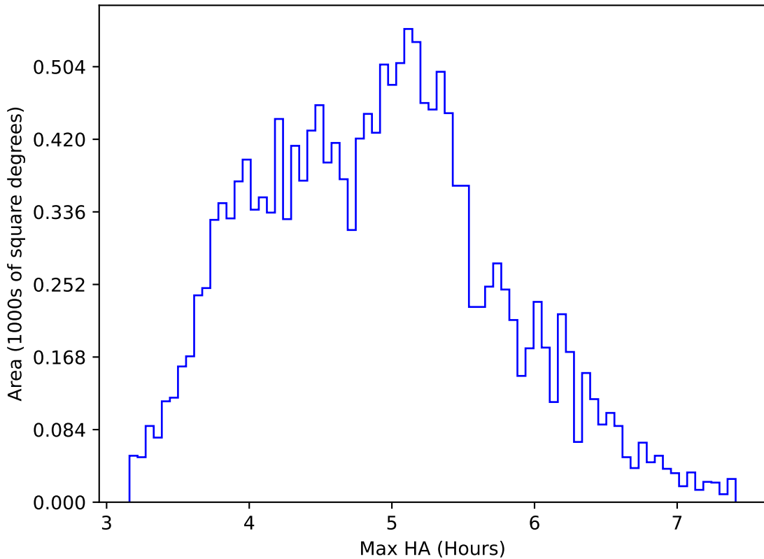
too_elab_r64_d2_griz_v3.4_10yrs WFD i band: Max HA
