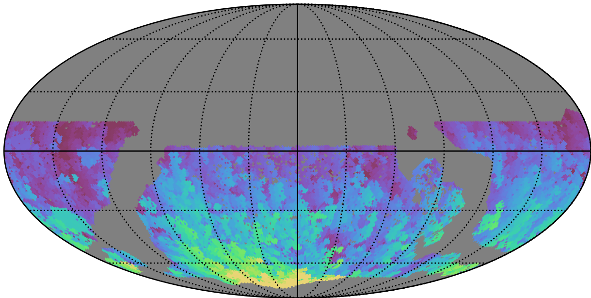
too_elab_r64_d2_griz_v3.4_10yrs WFD g band: Max HA
