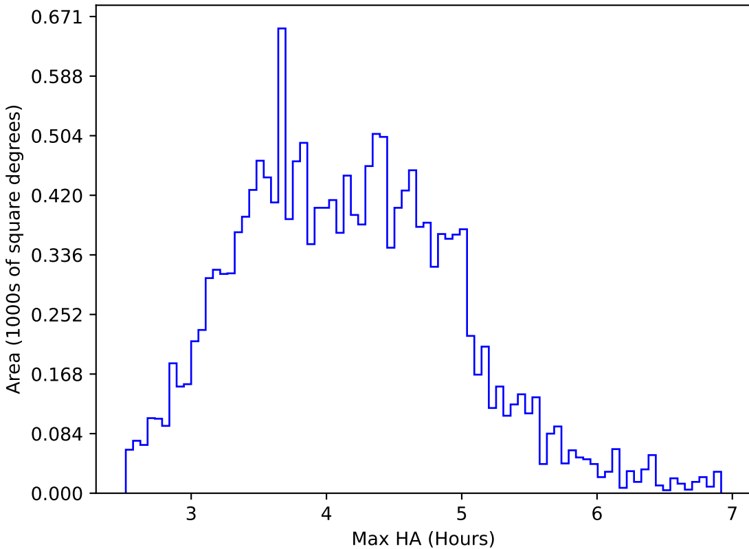
too_elab_r64_d2_griz_v3.4_10yrs WFD g band: Max HA
