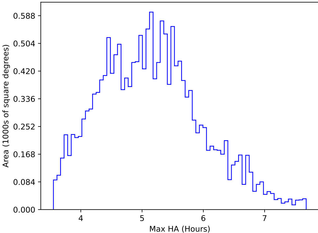
too_elab_r64_d2_griz_v3.4_10yrs WFD all bands: Max HA
