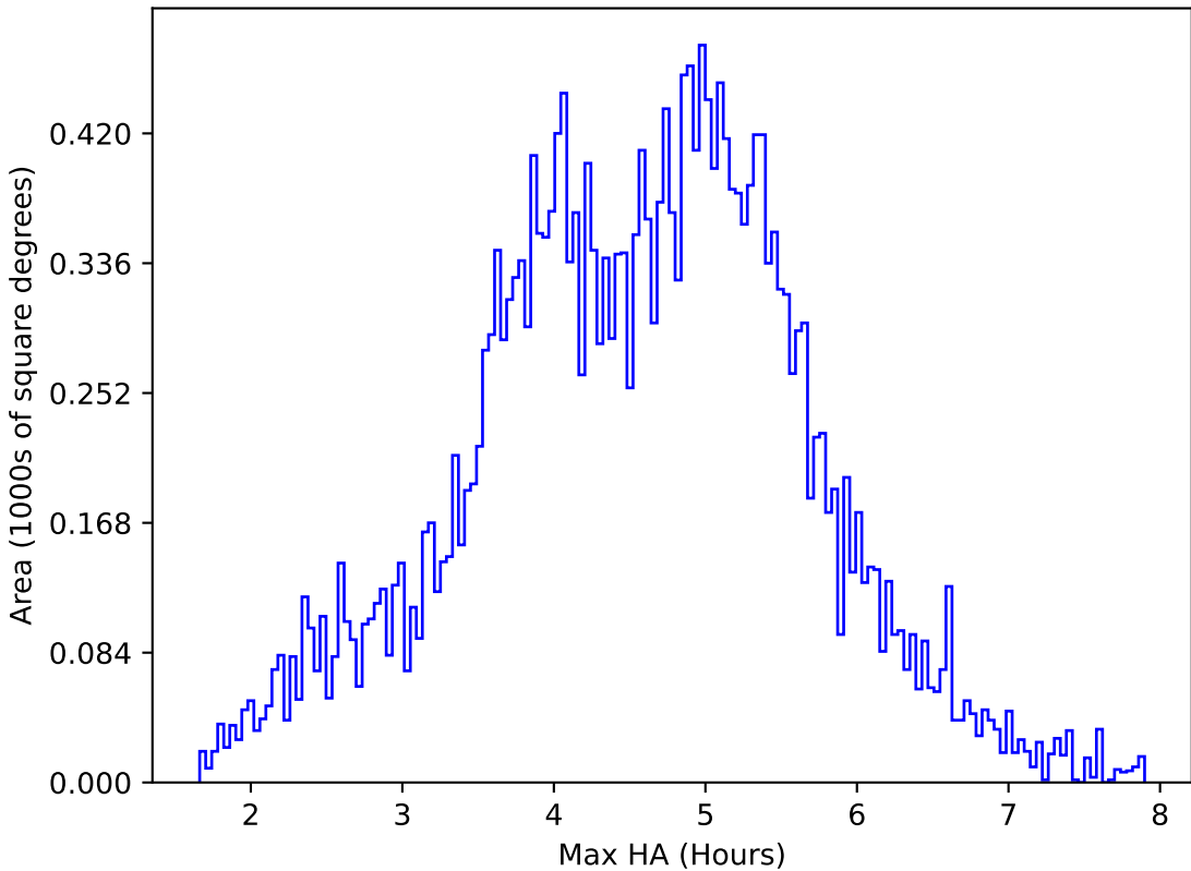
too_elab_r64_d2_griz_v3.4_10yrs All sky z band: Max HA
