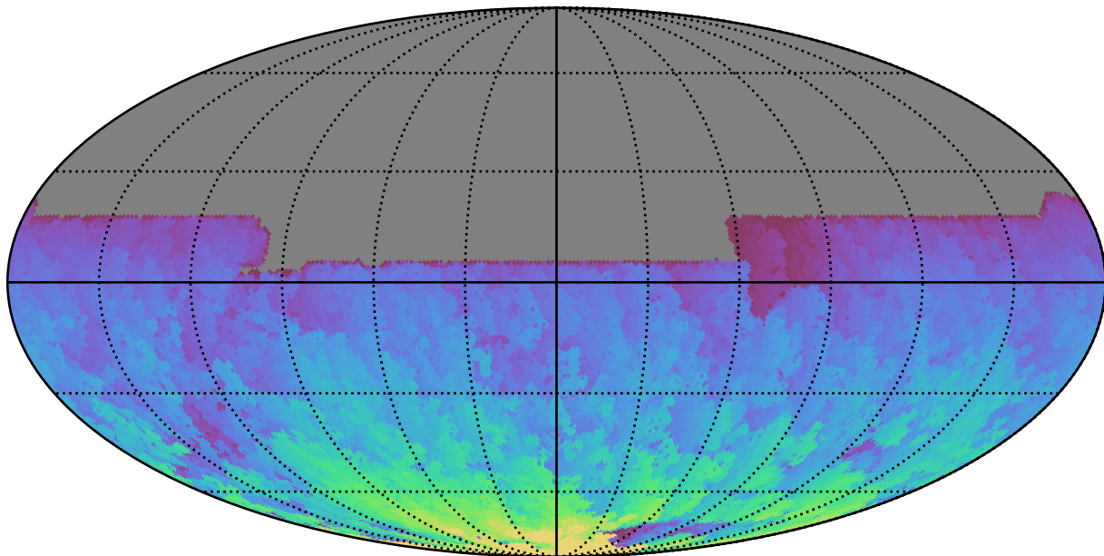
too_elab_r64_d2_griz_v3.4_10yrs All sky y band: Max HA
