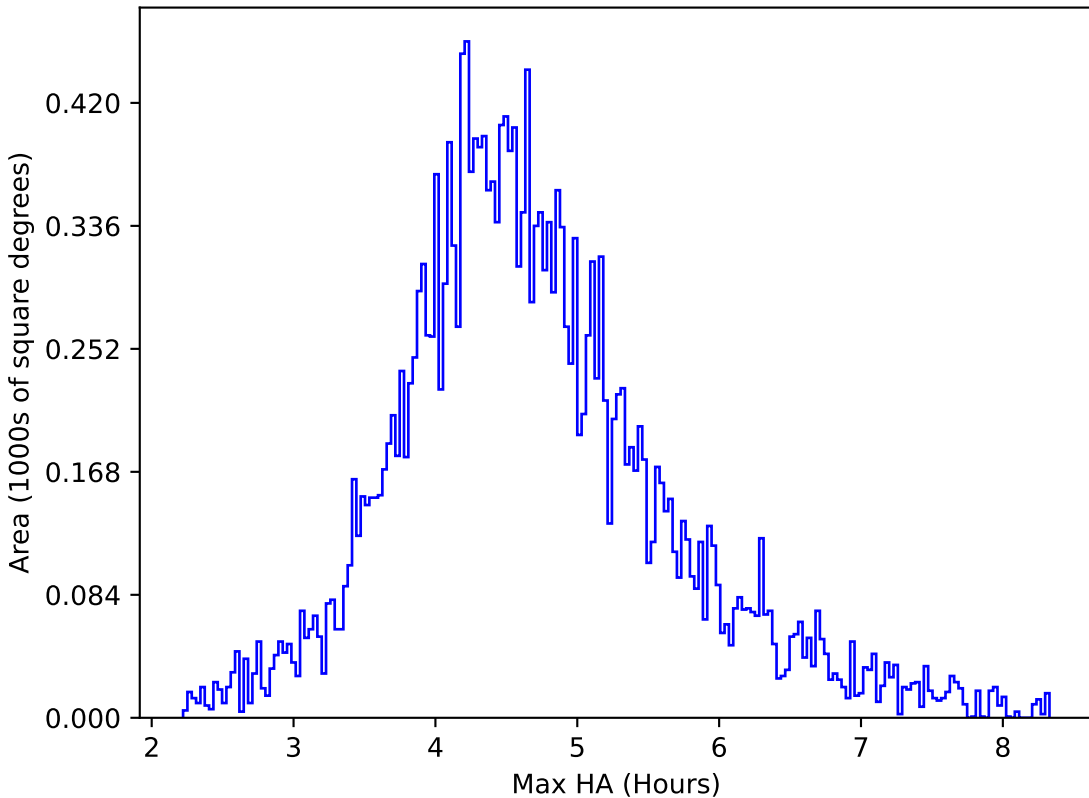
too_elab_r64_d2_griz_v3.4_10yrs All sky y band: Max HA
