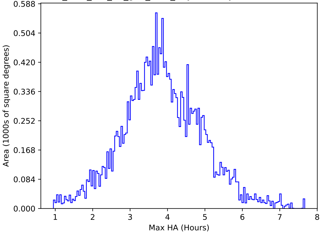
too_elab_r64_d2_griz_v3.4_10yrs All sky u band: Max HA
