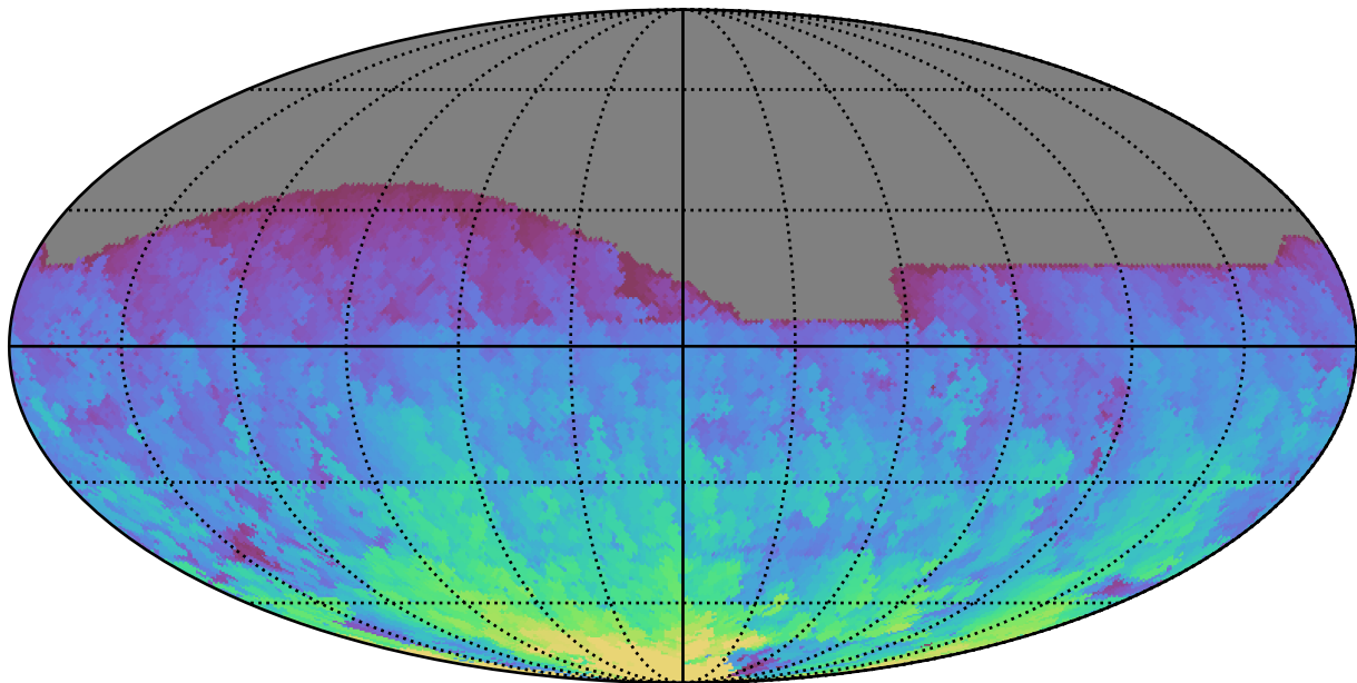
too_elab_r64_d2_griz_v3.4_10yrs All sky r band: Max HA
