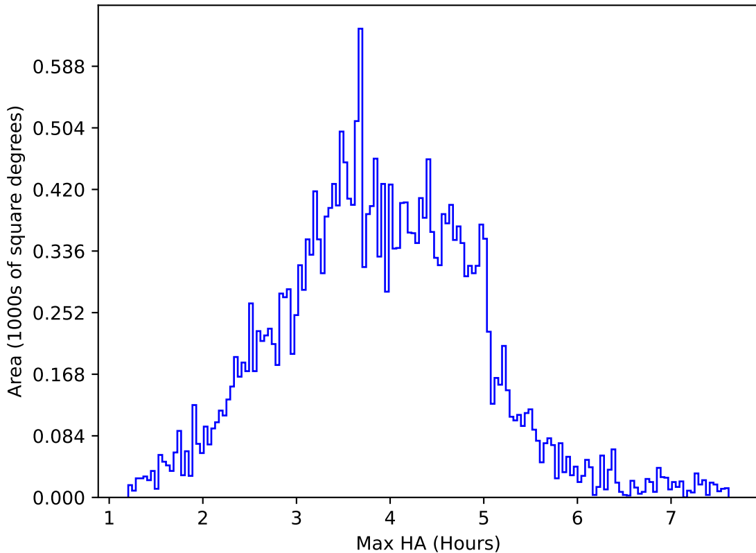
too_elab_r64_d2_griz_v3.4_10yrs All sky g band: Max HA
