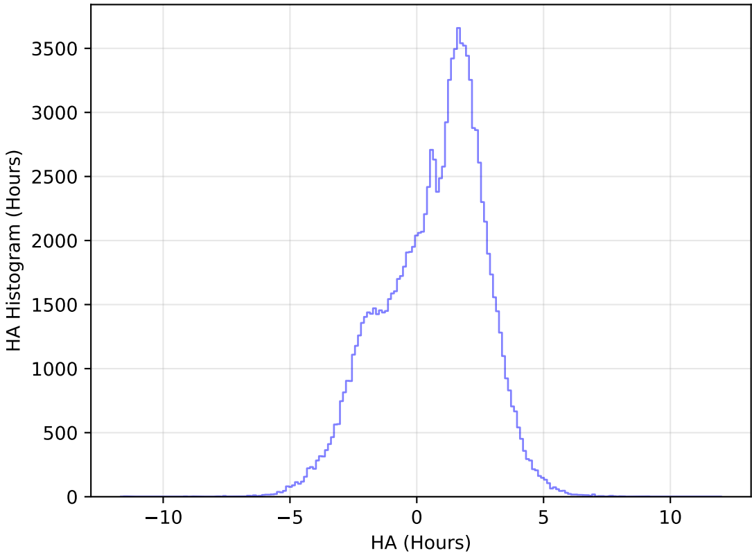
too_elab_r64_d2_griz_v3.4_10yrs WFD u band: HA Histogram
