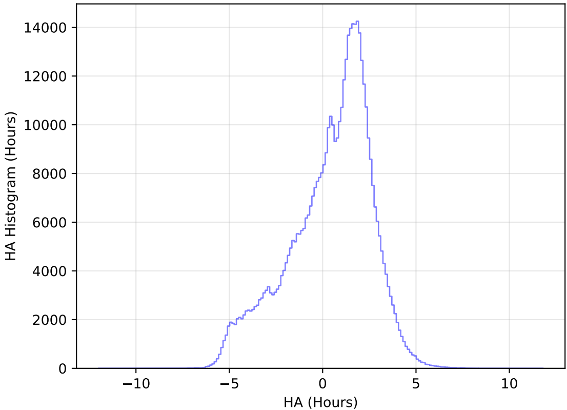
too_elab_r64_d2_griz_v3.4_10yrs WFD r band: HA Histogram
