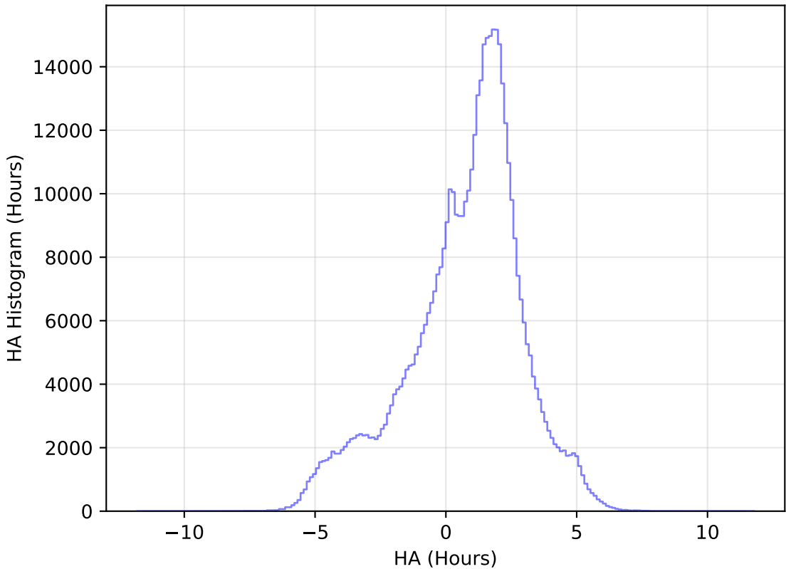
too_elab_r64_d2_griz_v3.4_10yrs WFD i band: HA Histogram
