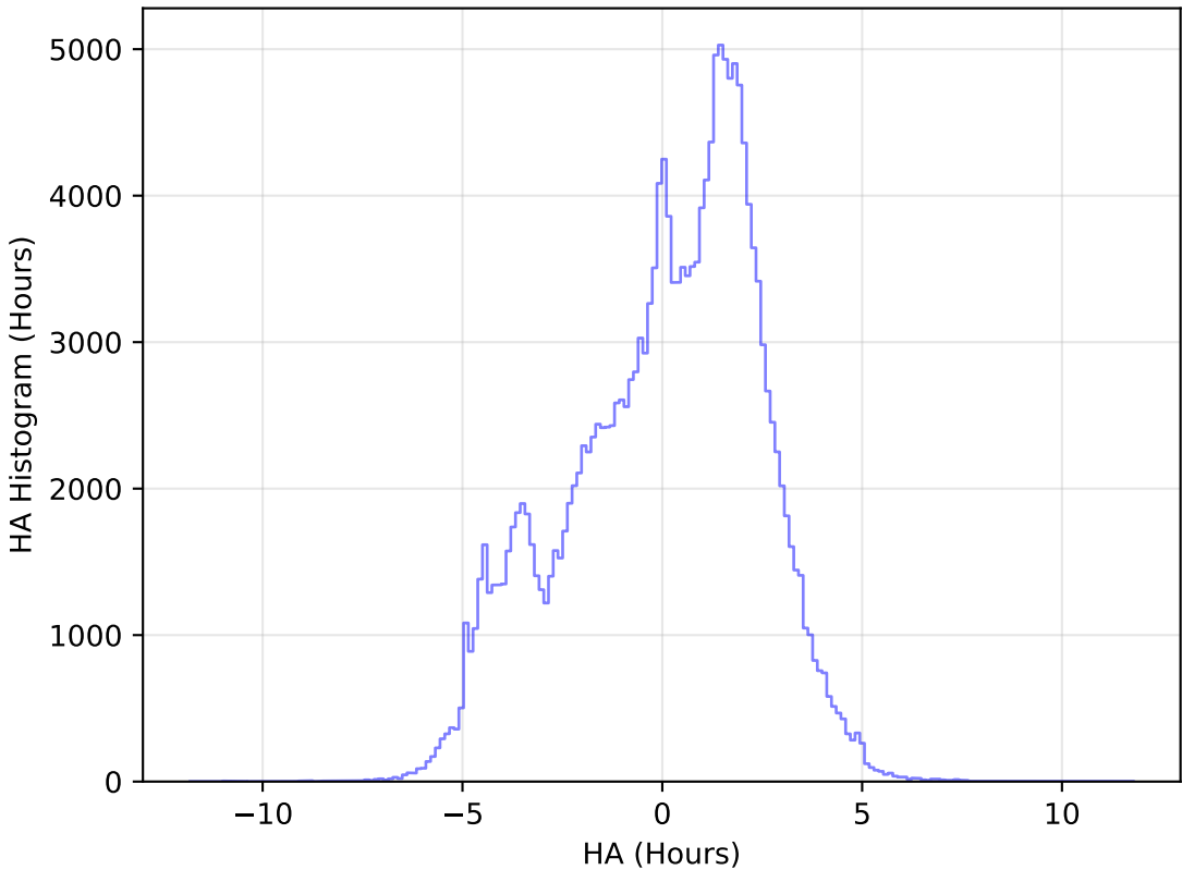
too_elab_r64_d2_griz_v3.4_10yrs WFD g band: HA Histogram
