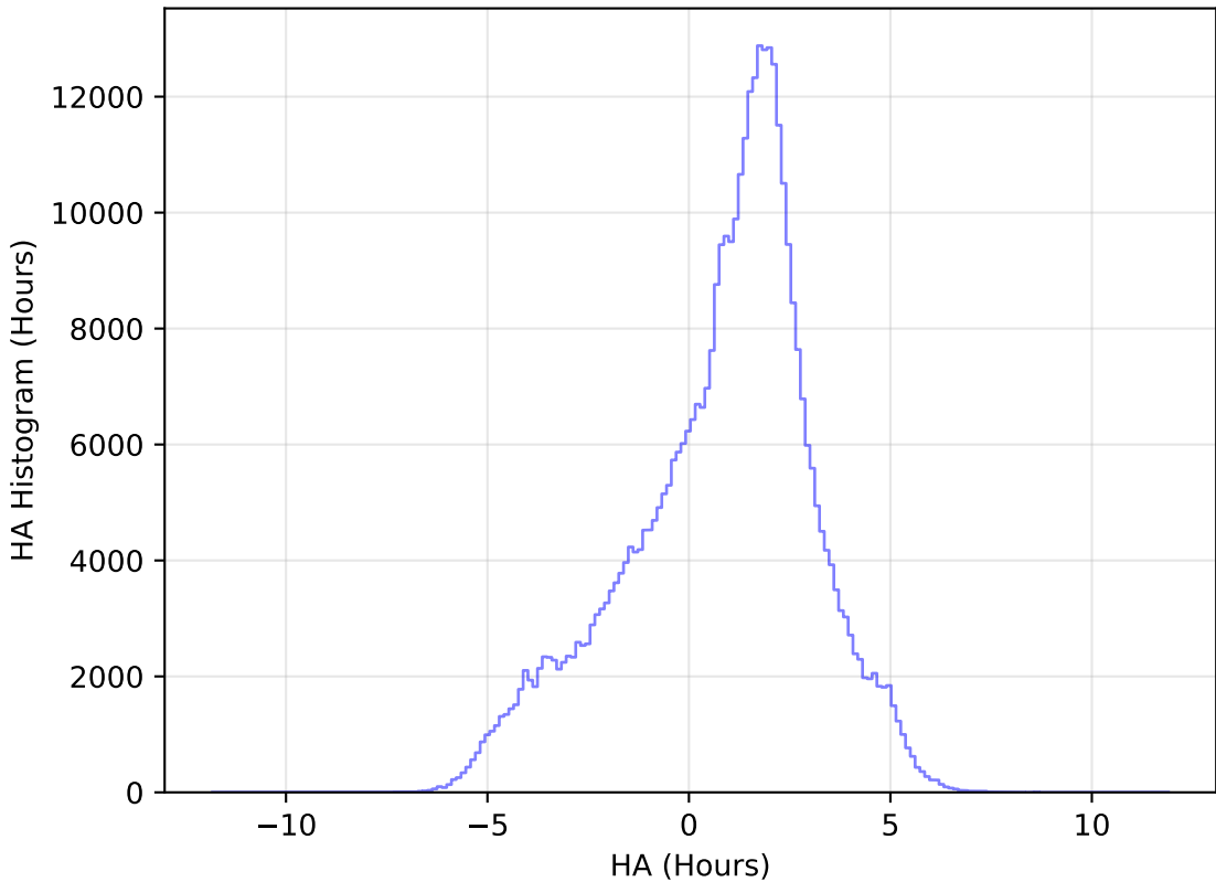
too_elab_r64_d2_griz_v3.4_10yrs All sky z band: HA Histogram
