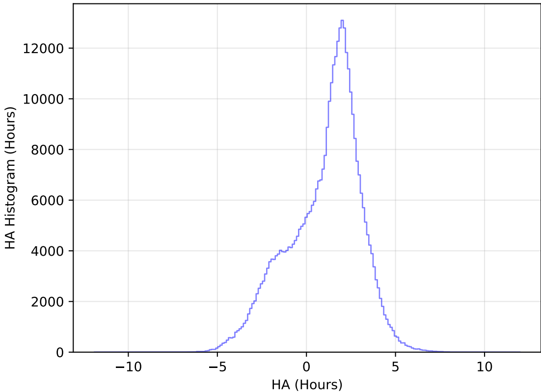
too_elab_r64_d2_griz_v3.4_10yrs All sky y band: HA Histogram
