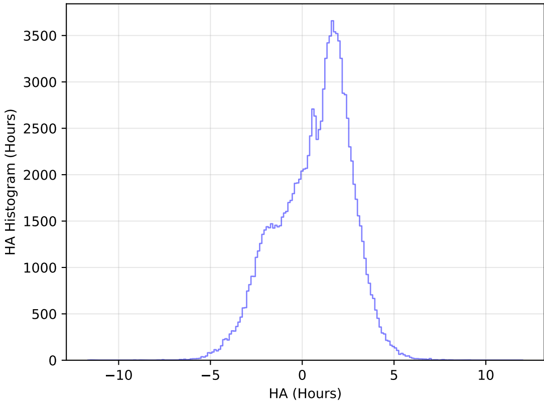
too_elab_r64_d2_griz_v3.4_10yrs All sky u band: HA Histogram
