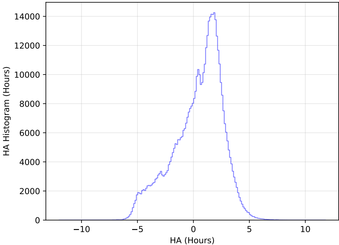
too_elab_r64_d2_griz_v3.4_10yrs All sky r band: HA Histogram
