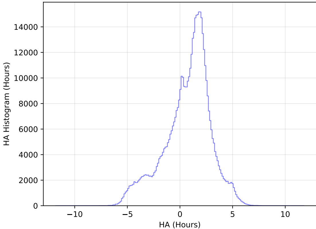
too_elab_r64_d2_griz_v3.4_10yrs All sky i band: HA Histogram
