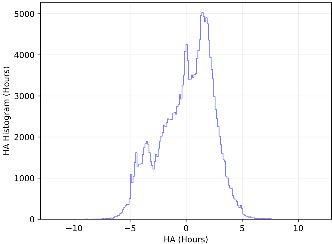
too_elab_r64_d2_griz_v3.4_10yrs All sky g band: HA Histogram
