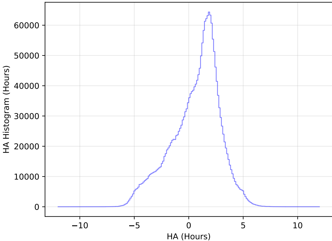
too_elab_r64_d2_griz_v3.4_10yrs All sky all bands: HA Histogram
