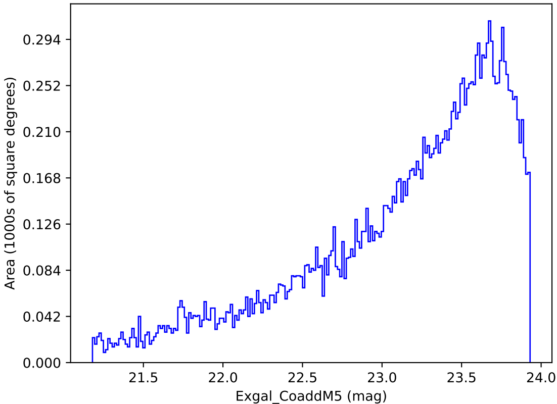
too_elab_r64_d2_griz_v3.4_10yrs Yr 3-4 y band: Exgal_CoaddM5
