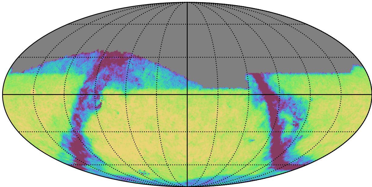
too_elab_r64_d2_griz_v3.4_10yrs Yr 1 i band: Exgal_CoaddM5
