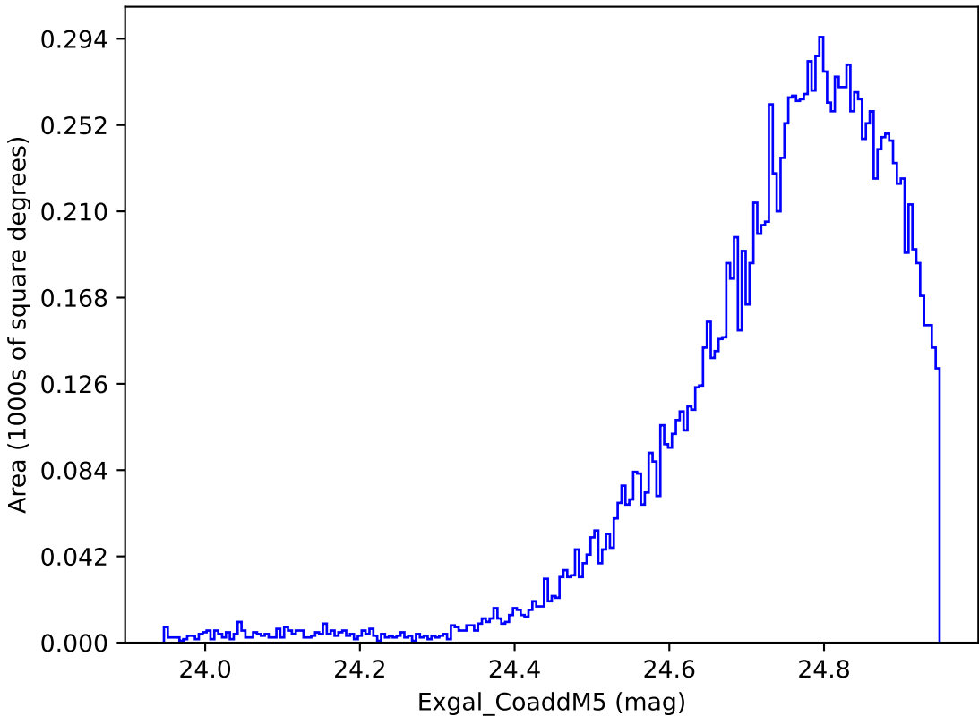
too_elab_r64_d2_griz_v3.4_10yrs WFD y band: Exgal_CoaddM5
