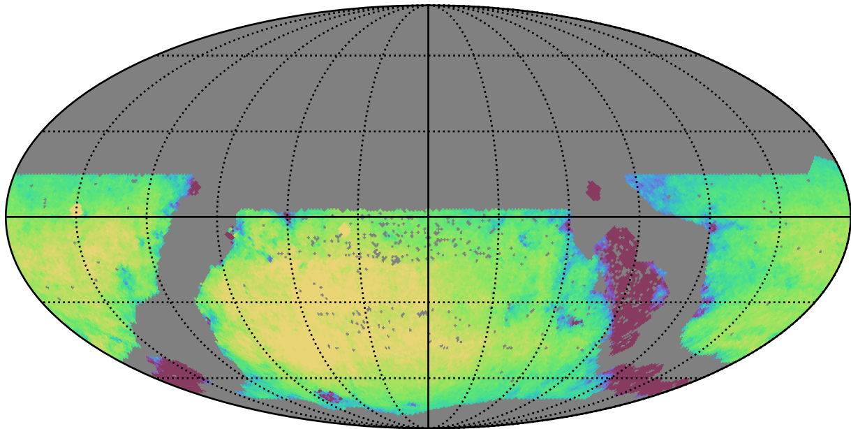
too_elab_r64_d2_griz_v3.4_10yrs WFD r band: Exgal_CoaddM5
