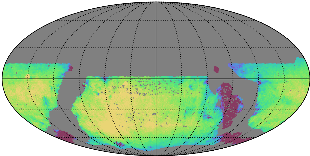
too_elab_r64_d2_griz_v3.4_10yrs WFD i band: Exgal_CoaddM5
