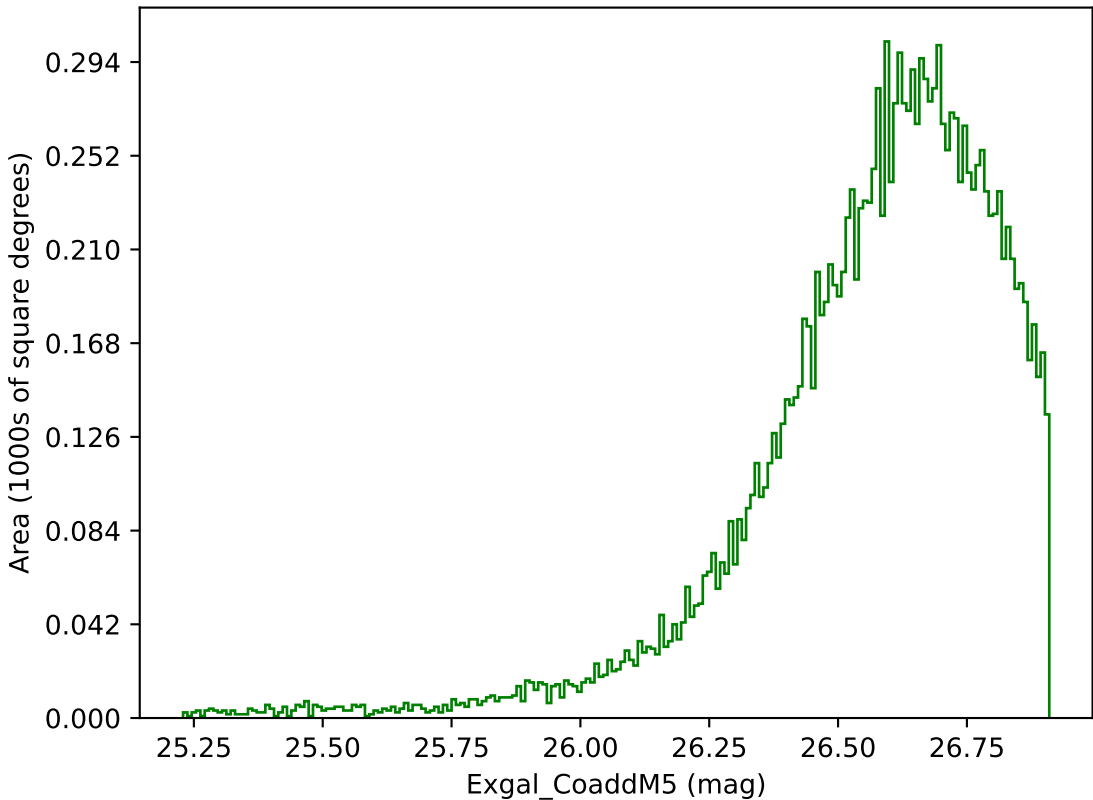
too_elab_r64_d2_griz_v3.4_10yrs WFD g band: Exgal_CoaddM5
