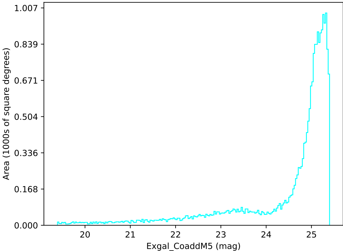
too_elab_r64_d2_griz_v3.4_10yrs All sky u band: Exgal_CoaddM5
