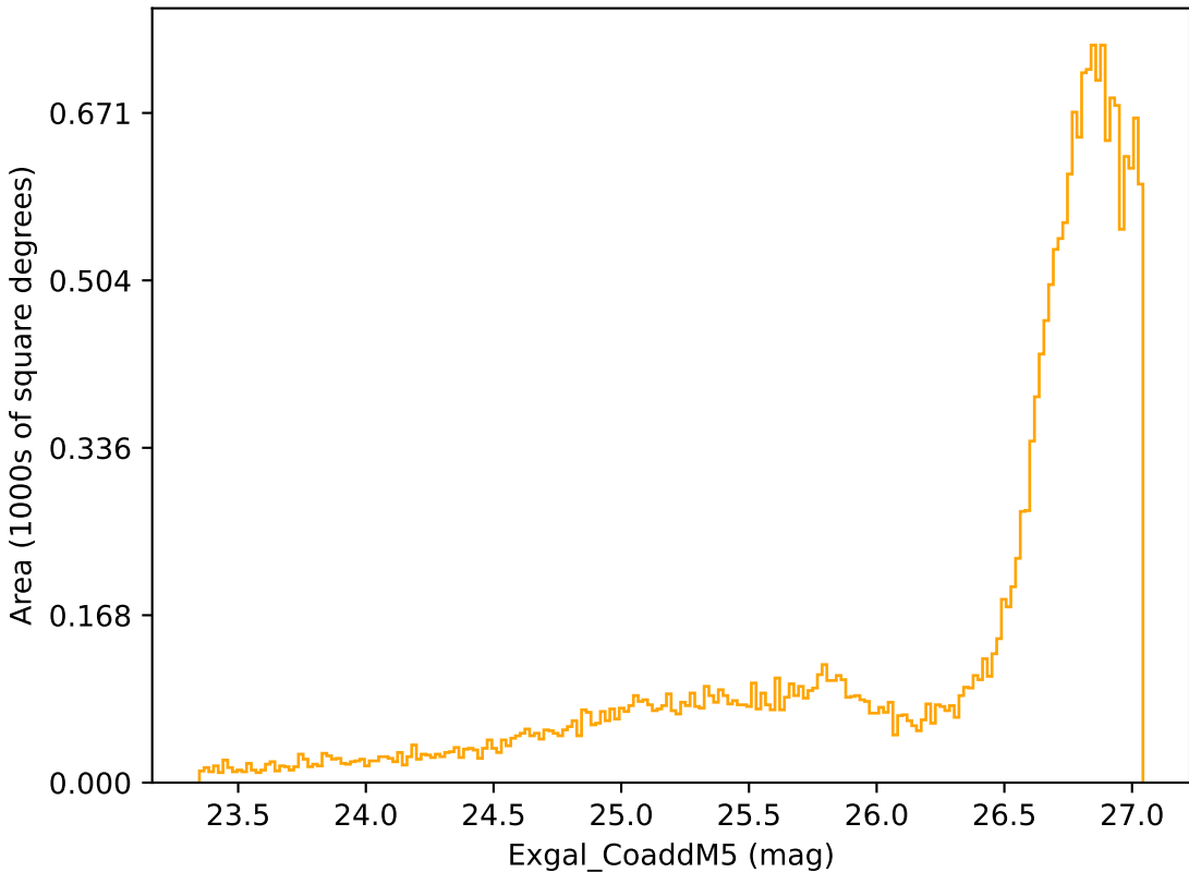
too_elab_r64_d2_griz_v3.4_10yrs All sky r band: Exgal_CoaddM5
