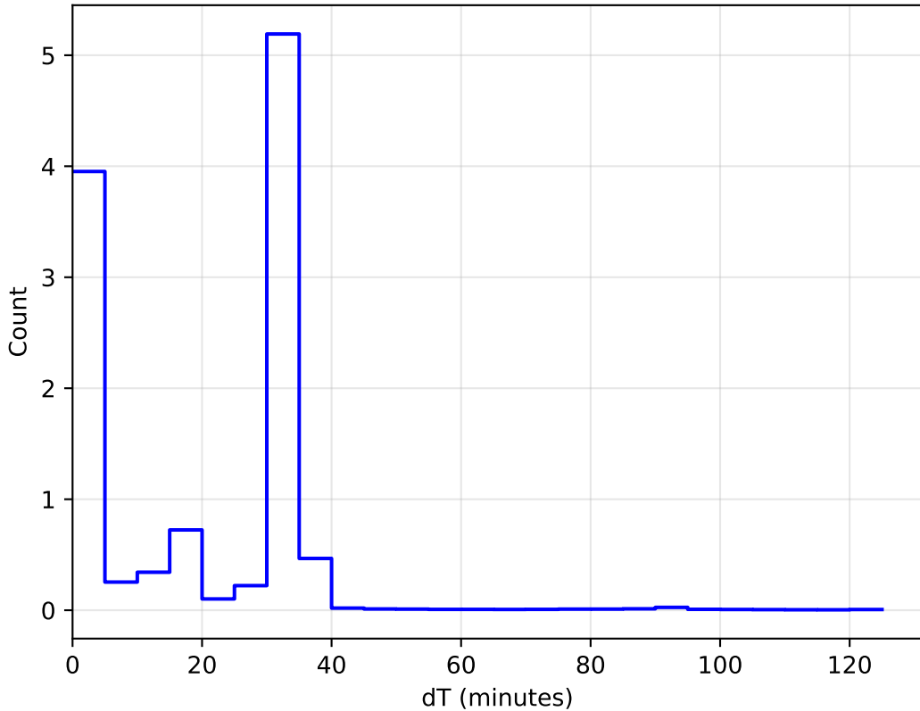
too_elab_r64_d2_griz_v3.4_10yrs WFD: DeltaT Histogram 1e6
