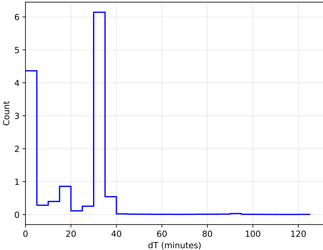
too_elab_r64_d2_griz_v3.4_10yrs All sky: DeltaT Histogram 1e6
