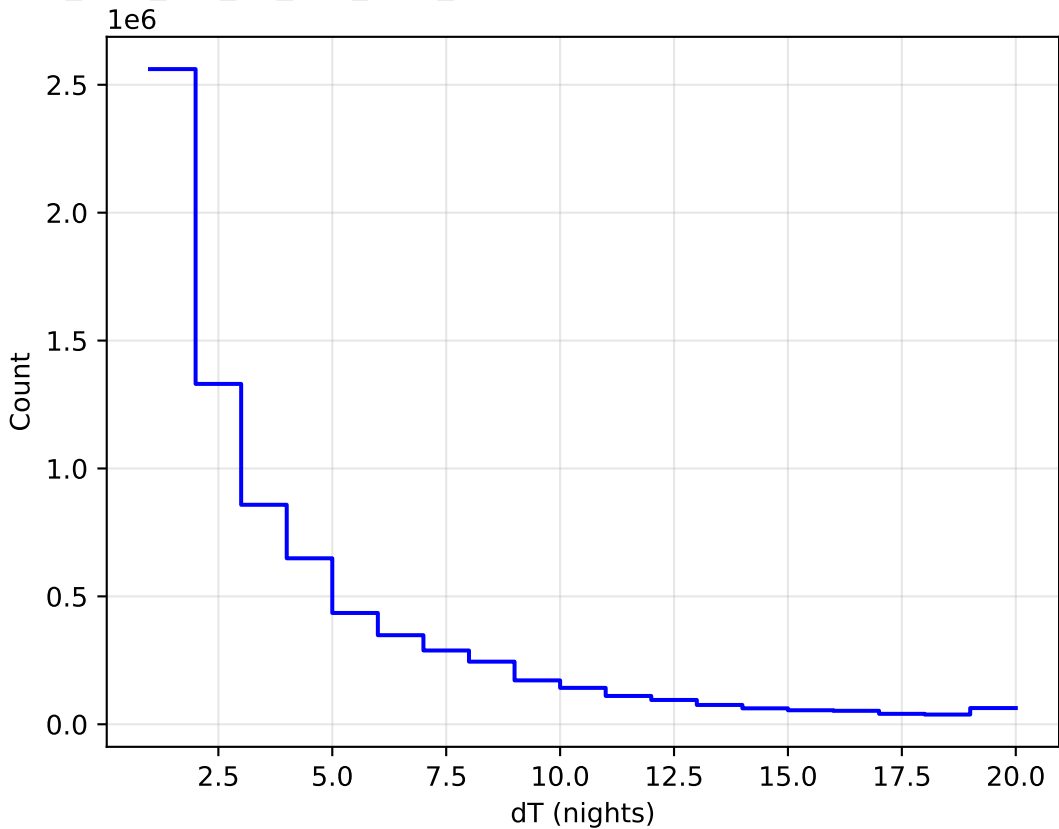
too_elab_r64_d2_griz_v3.4_10yrs WFD all bands: DeltaNight Histogram
