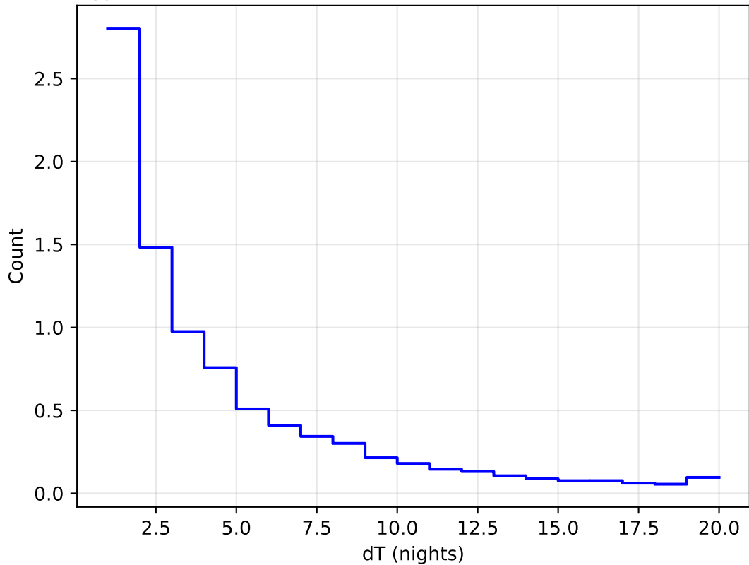
too_elab_r64_d2_griz_v3.4_10yrs All sky all bands: DeltaNight Histogram
