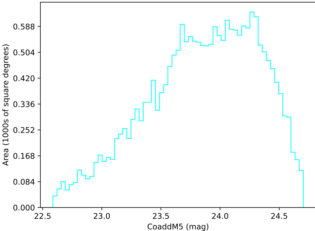
too_elab_r64_d2_griz_v3.4_10yrs Yr 3-4 u band: CoaddM5
