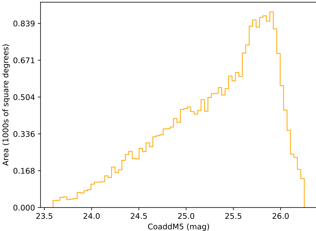
too_elab_r64_d2_griz_v3.4_10yrs Yr 3-4 r band: CoaddM5
