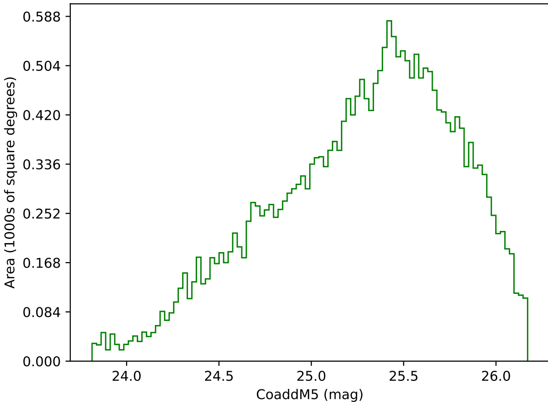
too_elab_r64_d2_griz_v3.4_10yrs Yr 3-4 g band: CoaddM5
