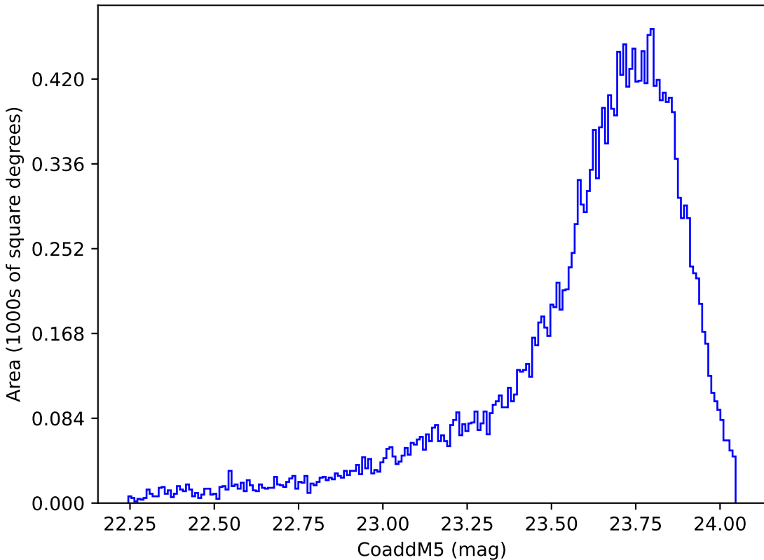
too_elab_r64_d2_griz_v3.4_10yrs Yr 1 y band: CoaddM5
