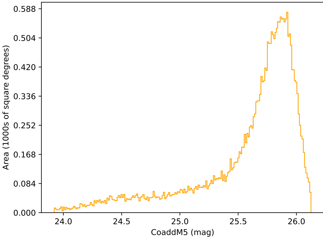
too_elab_r64_d2_griz_v3.4_10yrs Yr 1 r band: CoaddM5
