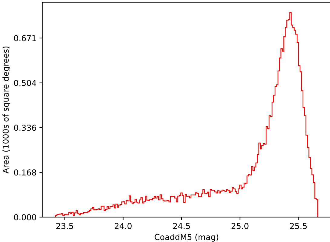
too_elab_r64_d2_griz_v3.4_10yrs Yr 1 i band: CoaddM5
